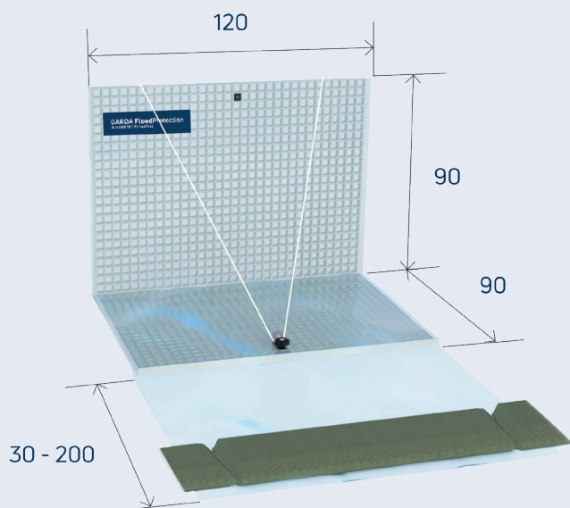
GARDA FloodProtection 90
