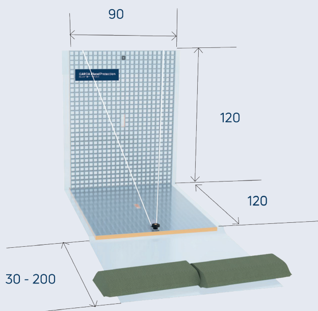
GARDA FloodProtection 120
